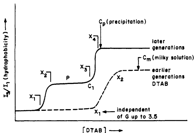
Figure 7. Schematic description of the dependence of I_3/I_1 on the concentration of DTAB in the presence of later generation (upper curve) and earlier generation (lower curve) starburst dendrimers.
